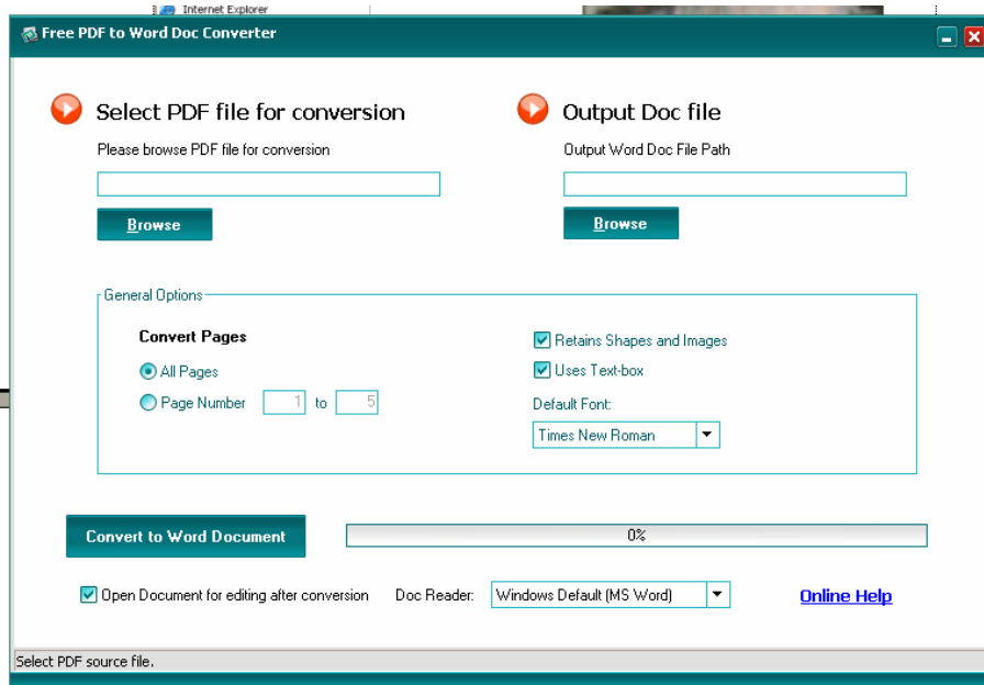
Gambar 10. Tampilan software
