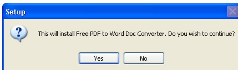
Gambar 2. Dialog penginstallan
