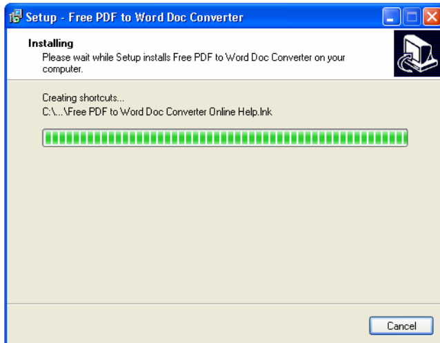
Gambar 7. Proses pengintallan
