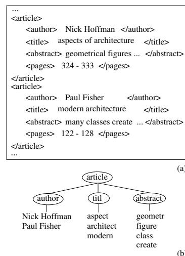
Figure 2: (a) An XML document and (b) its Summary tree
