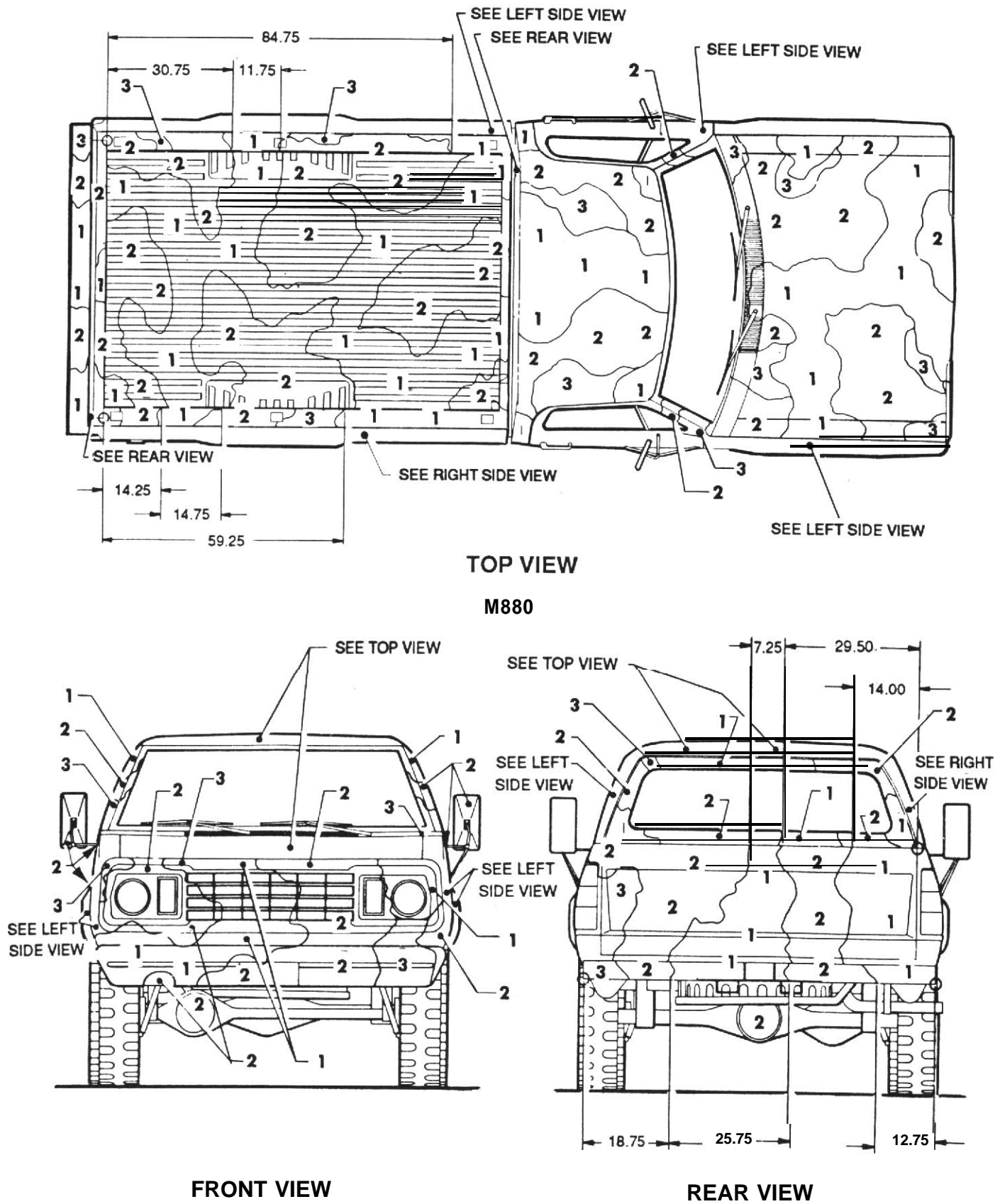
Figure 36. Truck, cargo: 1-1/4-ton M880. (1 of 2)
