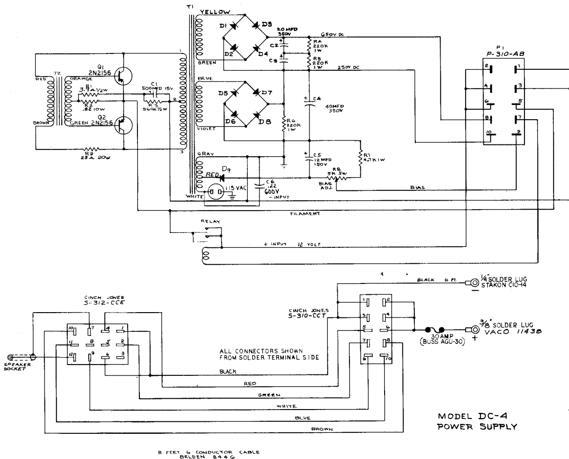
Figure 5-5. Power Supply Schematic Diagrams
