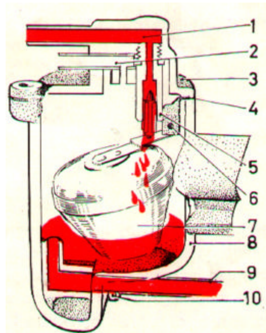
Fig. 80 Spring-loaded needle suspension
