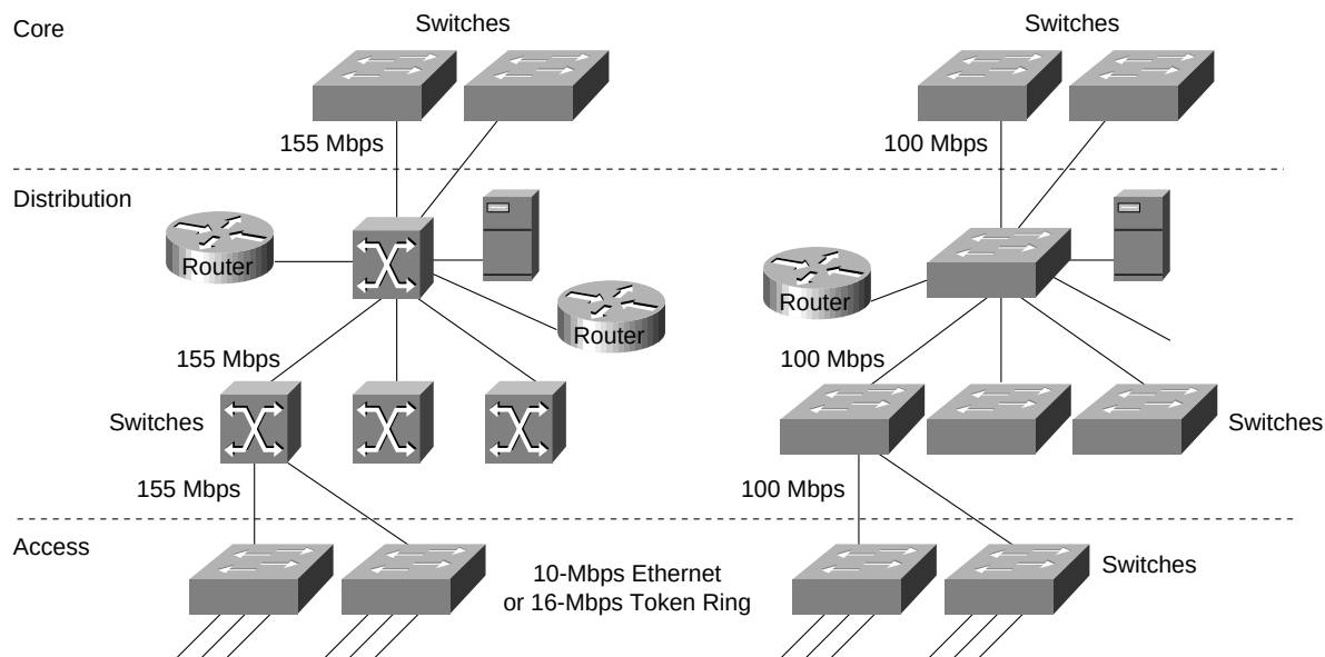
Figure 12-15 Large switched/minimal routing design.
