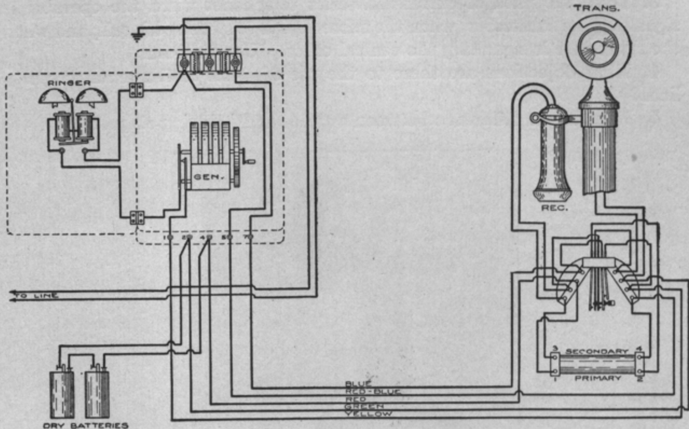
Desk telephone wired for series operation.
