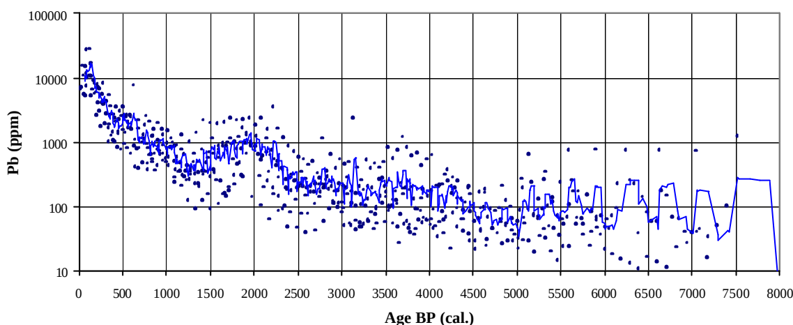
Fig. 1 The distribution of lead (Pb) in the 10 bogs investigated
