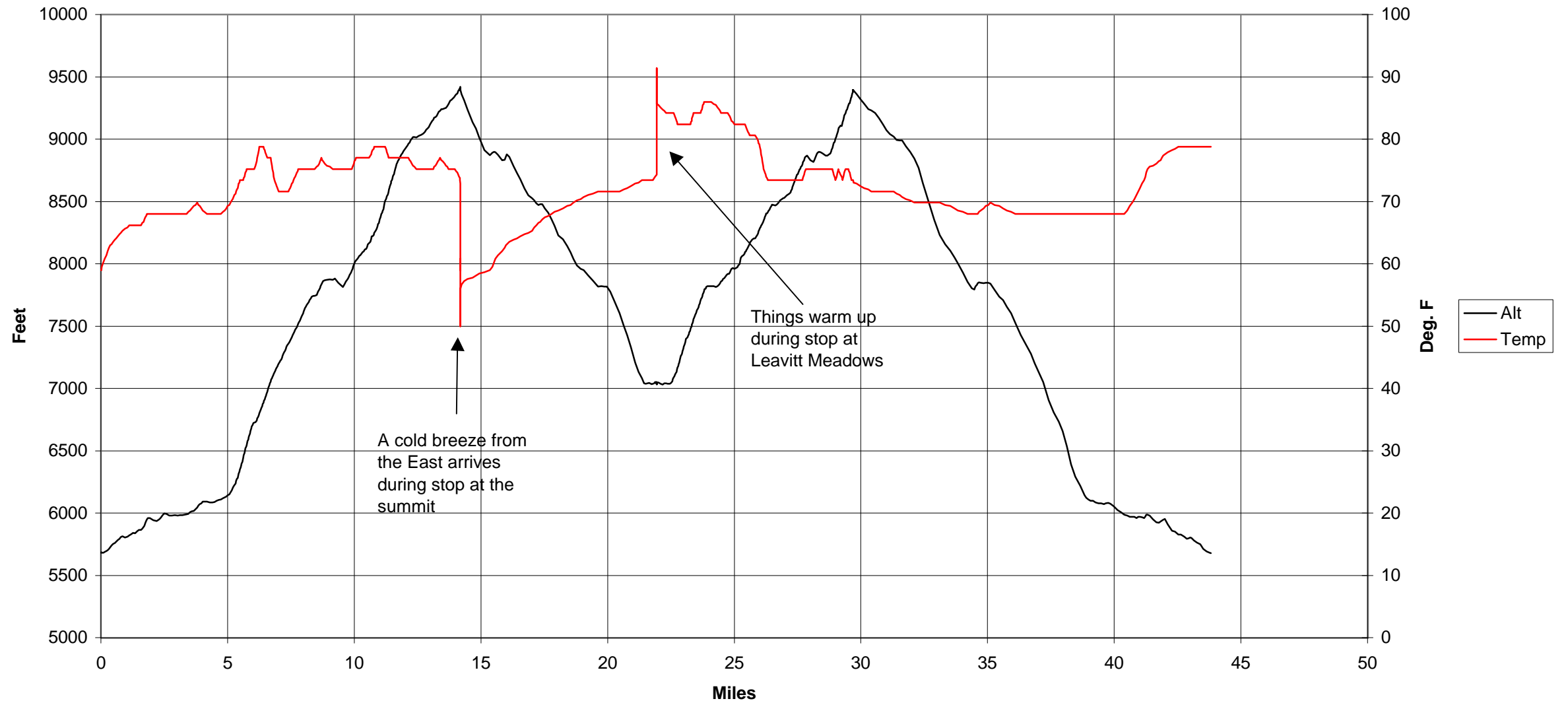
Elevation and Air Temperature v. Miles
