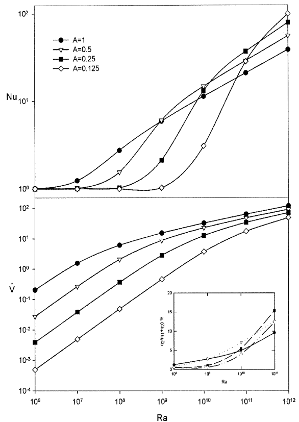
Fig. 6. Normalized Nusselt number and volume flow rate as a function of Rayleigh number with the aspect ratio as a parameter for the case with \ell/L = 0.10 , k_r = 20 , \varphi = 90^\circ .
