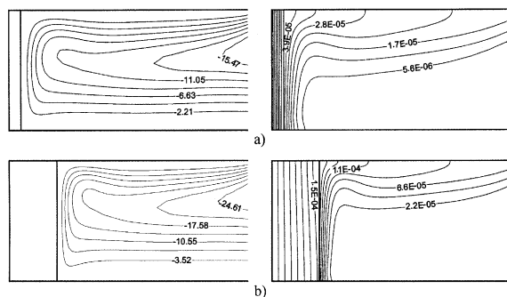
Fig. 4. Streamlines (on the left) and isotherms (on the right) for the case of A = 0.5 , k = 20 , \varphi = 90^\circ and Ra = 10^{10} , and various \ell/L : (a) \ell/L = 0.05 , (b) \ell/L = 0.20 .
