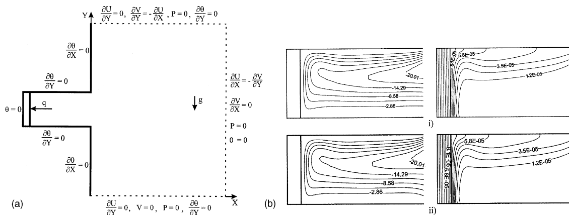
Fig. 2. Comparison study with extended computational domain: (a) schematic of extended domain, (b) streamlines and isotherms for the base case at Ra = 10^{10} using (i) restricted domain, (ii) extended domain.
