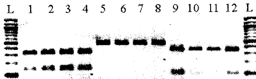
Fig. 4. Hae III restriction enzyme pattern for 12 sandhill cranes, lanes 1–4 = group C (greater); lanes 5–8 = group B (Canadian and greater), lanes 9–12 = group A (lesser). Groups B and C are not phylogenetically distinct, and thus can be combined (see text for details). L = 100 base pair (bp) Ladder (New England Biolabs, Beverly, Massachusetts, USA); bands beginning at the bottom correspond to 100, 200, 300, 400, 500, 600, 700, 800, 900, 1000, 1200, and 1500 bp. The 500 and 1000 bp bands of the ladder have larger amounts of DNA, obscuring the 900 bp band under the gel conditions used.
