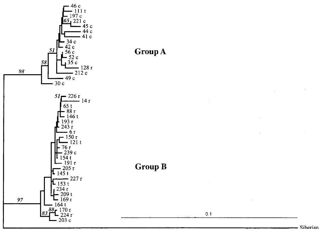
Fig. 3. Rooted phylogram showing that the sandhill crane mtDNA sequences fall into 2 groups. Tree was constructed from Hasegawa-Kishino-Yano (HKY85; 1985) genetic distances using the Neighbor Joining algorithm of PAUP* 4.0b2a (Swofford 1999). Siberian crane was used as an outgroup and demonstrates interspecific differentiation. Bootstrap values \geq 50\% are given above the branches. Numbers refer to the individual identifications. Letters following the numbers represent the first letter of subspecies, determined by morphological analysis [c = Grus canadensis canadensis (lesser), r = G. c. rowani (Canadian), t = G. c. tabida (greater)].
