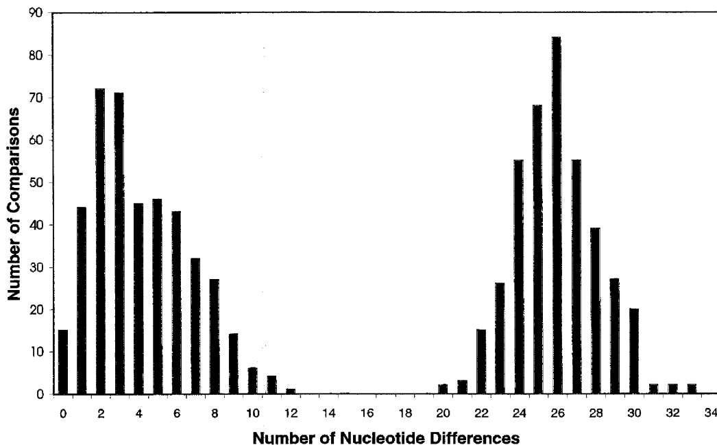
Fig. 2. Distribution of nucleotide differences among mtDNA haplotypes of sandhill cranes.
