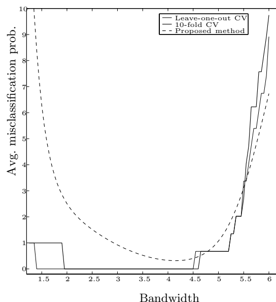
Figure 3.2. Average misclassification probabilities (Wine Data).
