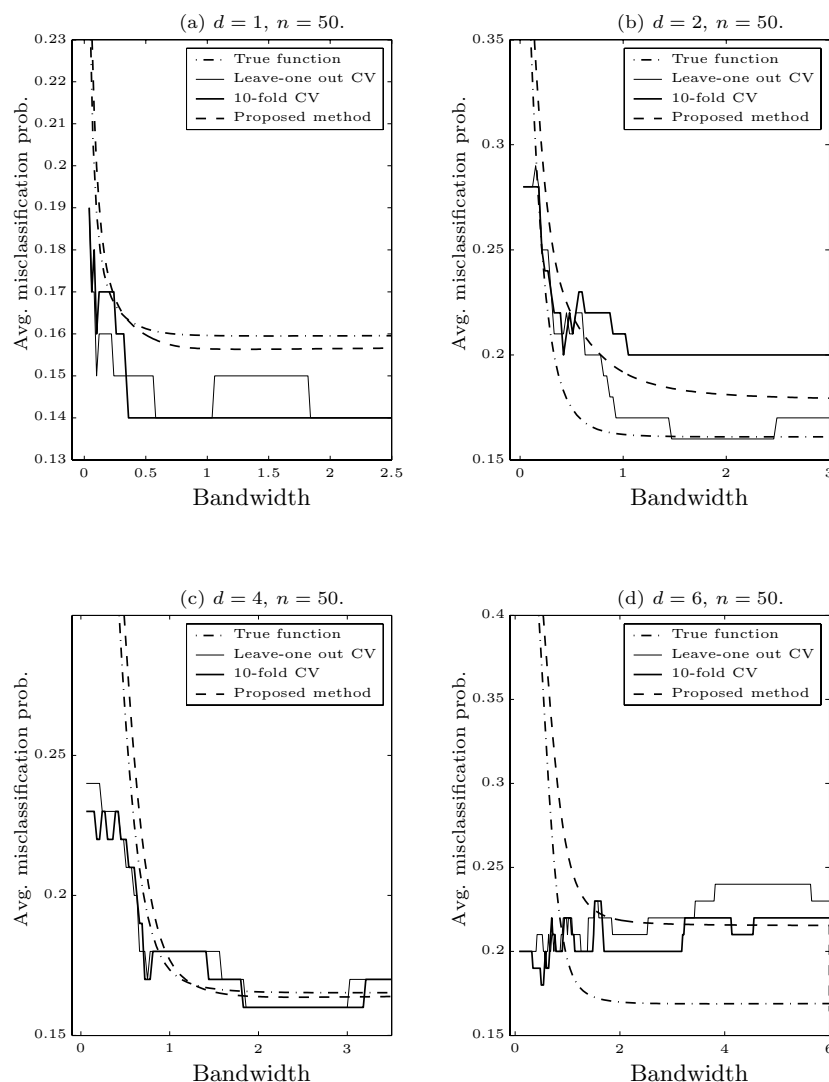
Figure 1.2. Average misclassification probabilities (equal prior cases).
