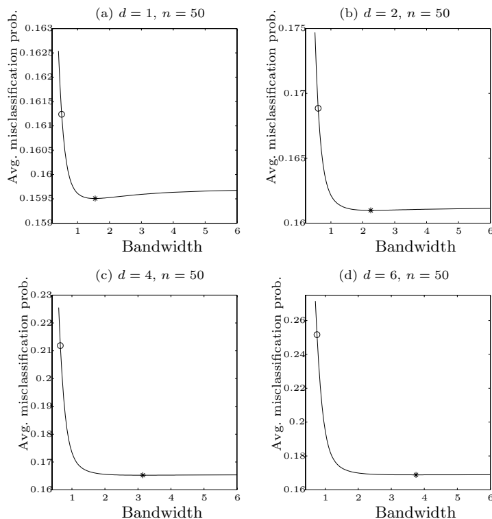
Figure 1.1. True \Delta -function and optimal bandwidths (equal prior cases).
