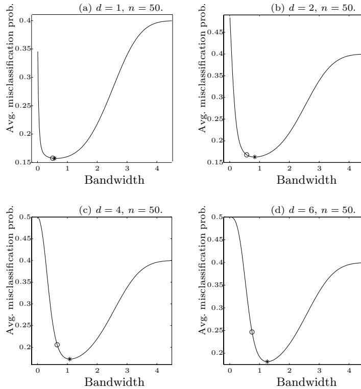
Figure 2.1. True \Delta -function and optimal bandwidths (unequal prior cases).
