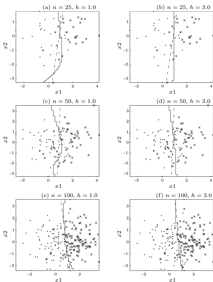
Figure 2.3. Classification boundaries for fixed bandwidth kernel classifiers and linear classifiers.
