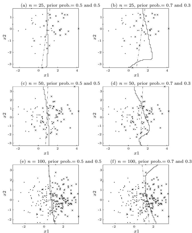
Figure 2.2. Classification boundaries for kernel based and linear classifiers.
