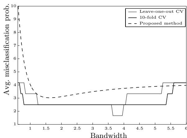
Figure 3.1. Average misclassification probabilities (Iris Data).
