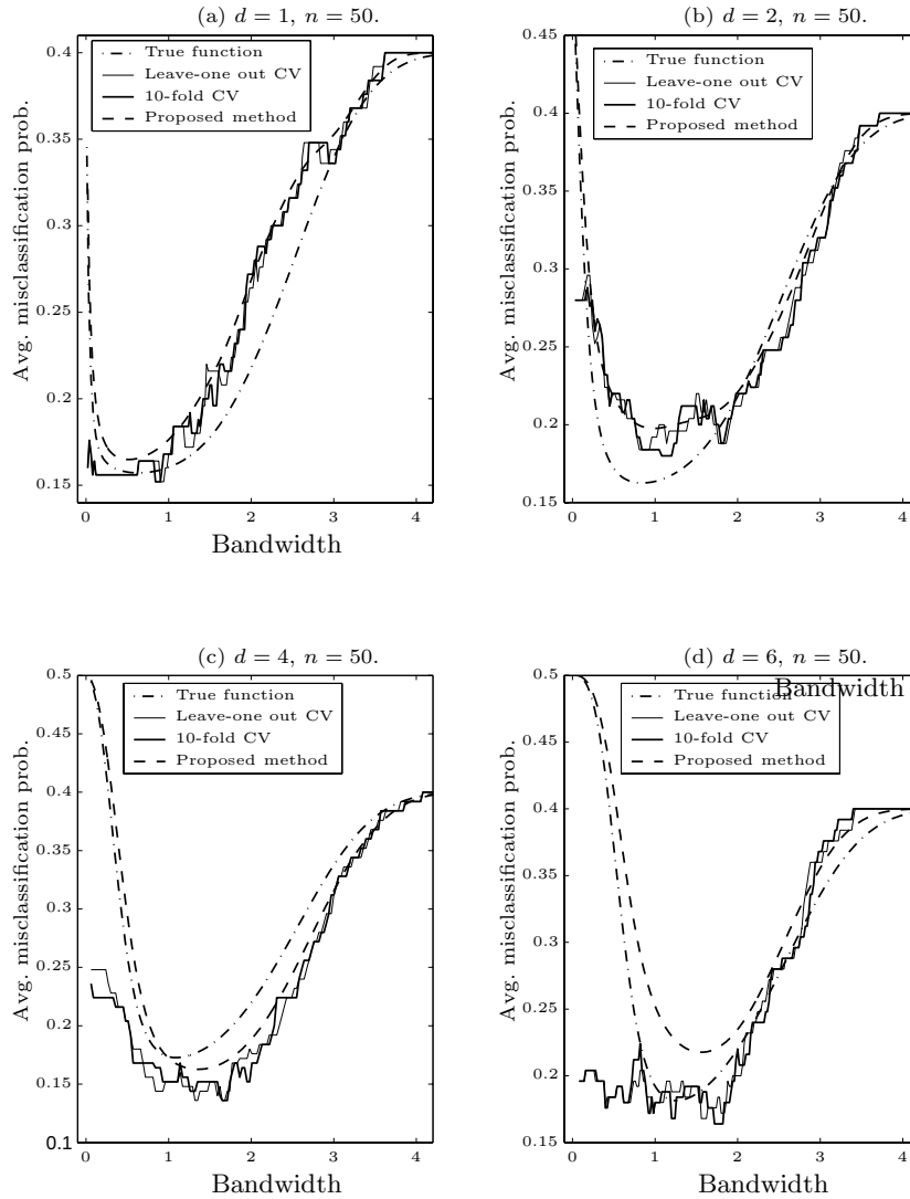
Figure 2.4. Average misclassification probabilities (unequal prior cases).
