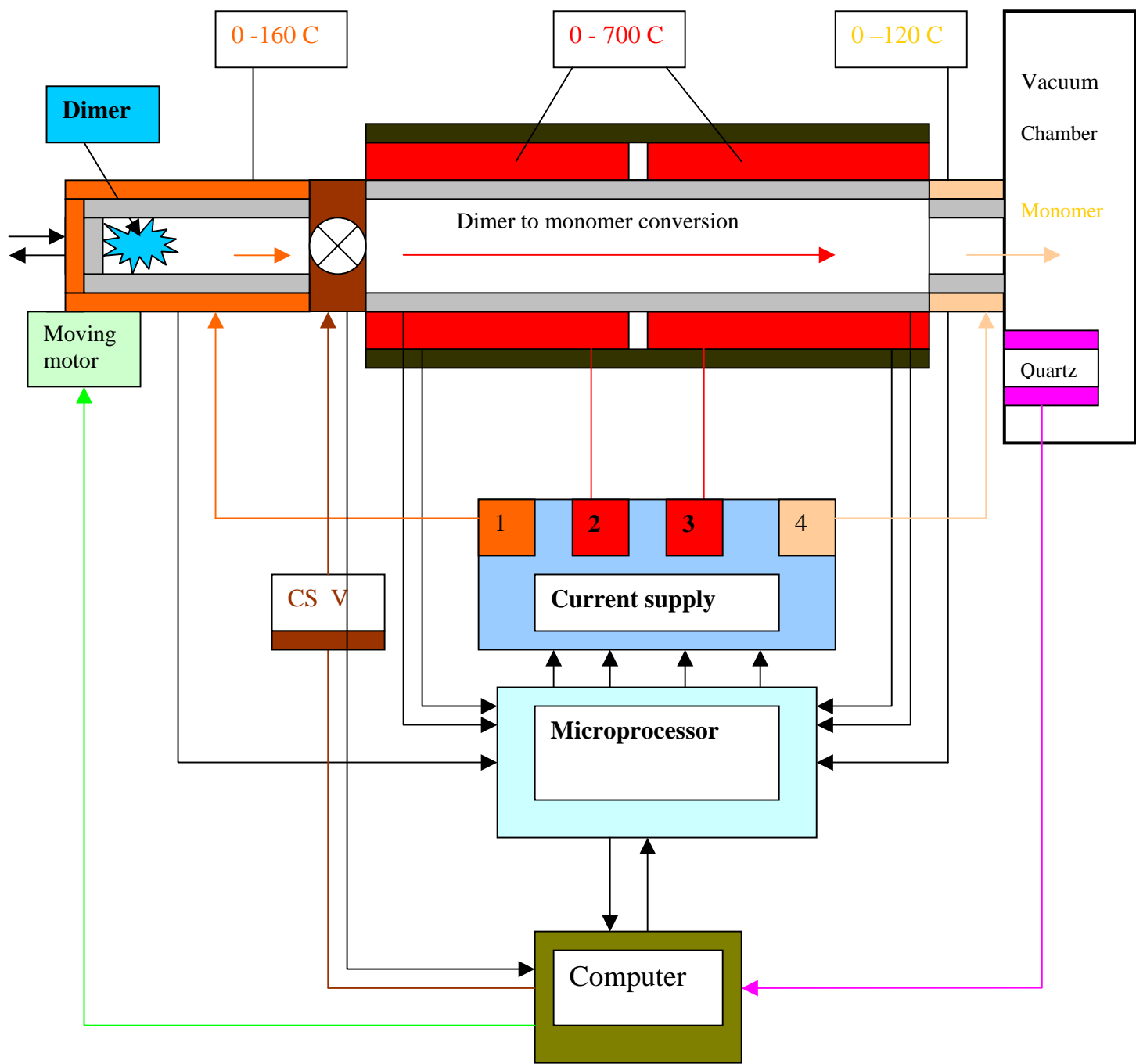
Scheme of the installation for the dimer evaporation, conversion to monomer and controlled supply to vacuum chamber for deposition of POLYPARAXYLYLENE films.
