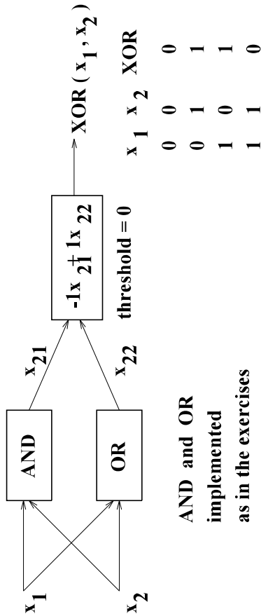
Figure 4.19: Implementation of XOR using a feedforward ANN
