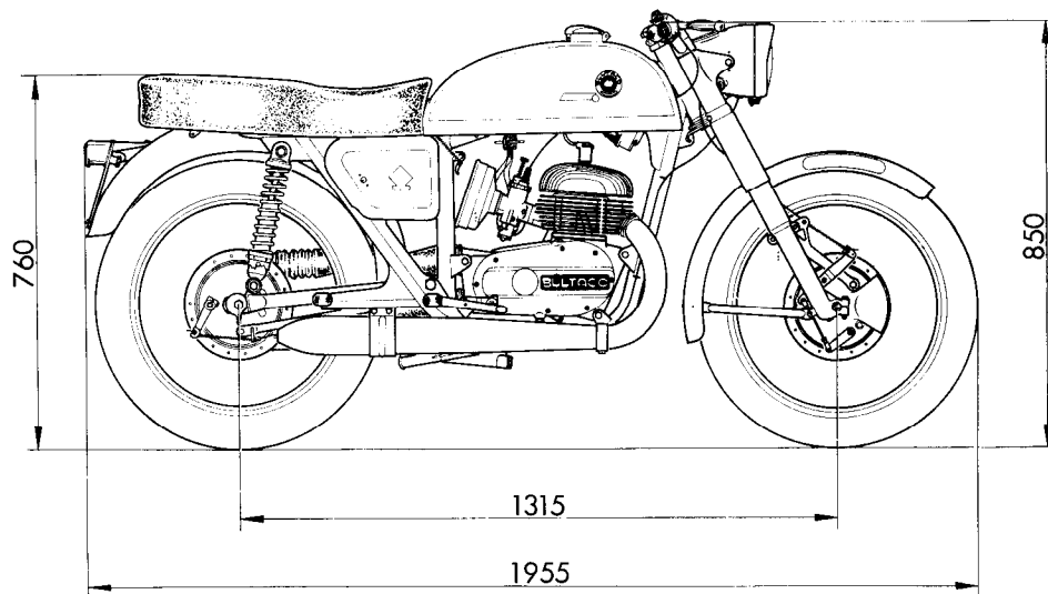
Fig. 36. — Overall dimensions.
