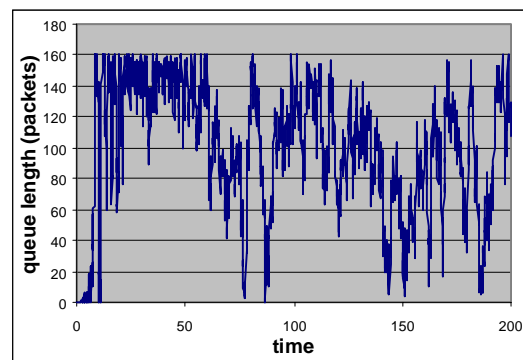
Figure 15. BLUE queue size graph for q_{\max} = 160 (large RTT)
