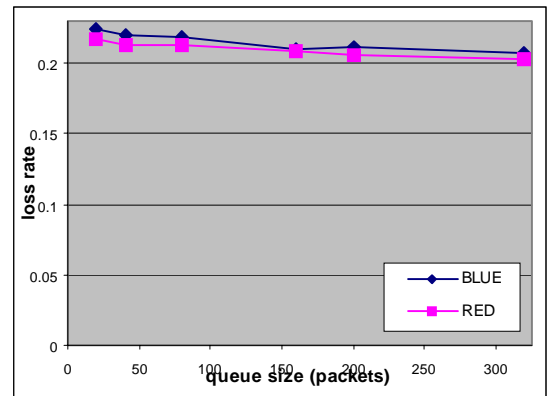
Figure 13. Total drop rate over bottleneck link for both RED and BLUE (large RTT, without ECN)
