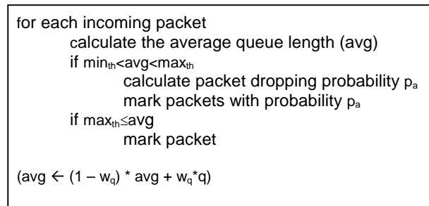
Figure 1. RED Algorithm
