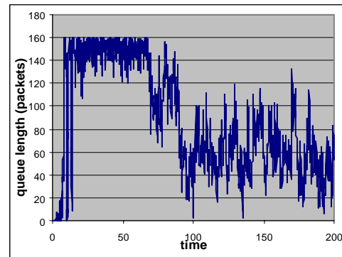
Figure 7. Queue size for BLUE when q\_max = 160 (large RTT)
