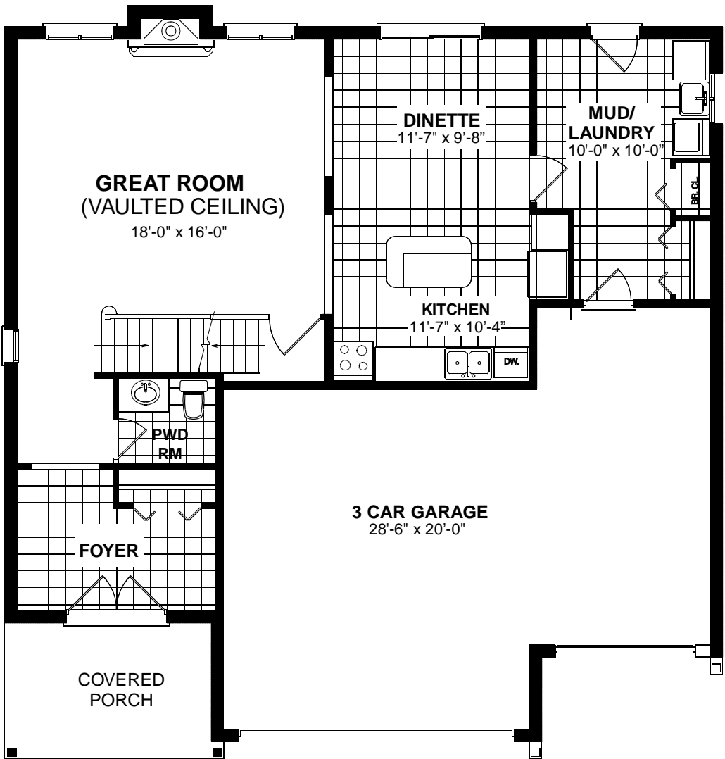
MAIN FLOOR PLAN 1404 SQ. FT.
