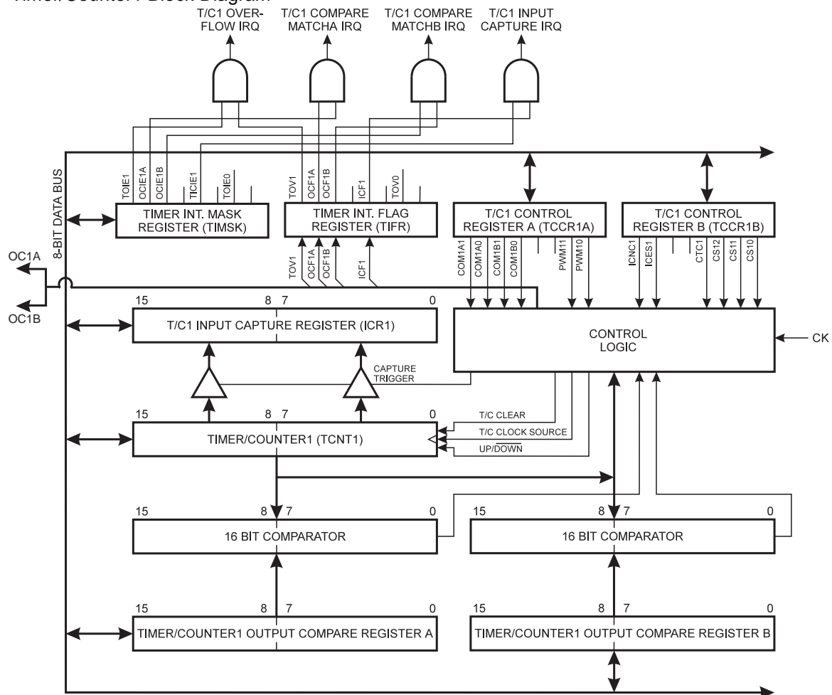
Figure 3. Timer/Counter1 Block Diagram
