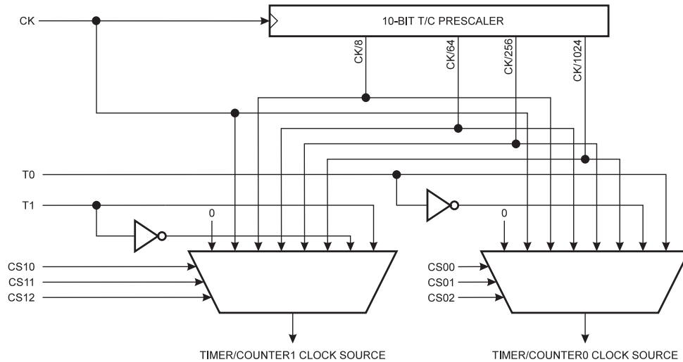
Figure 1. Timer/Counter Prescaler.
