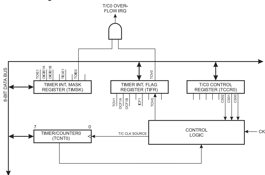
Figure 2. Timer/Counter0 Block Diagram.
