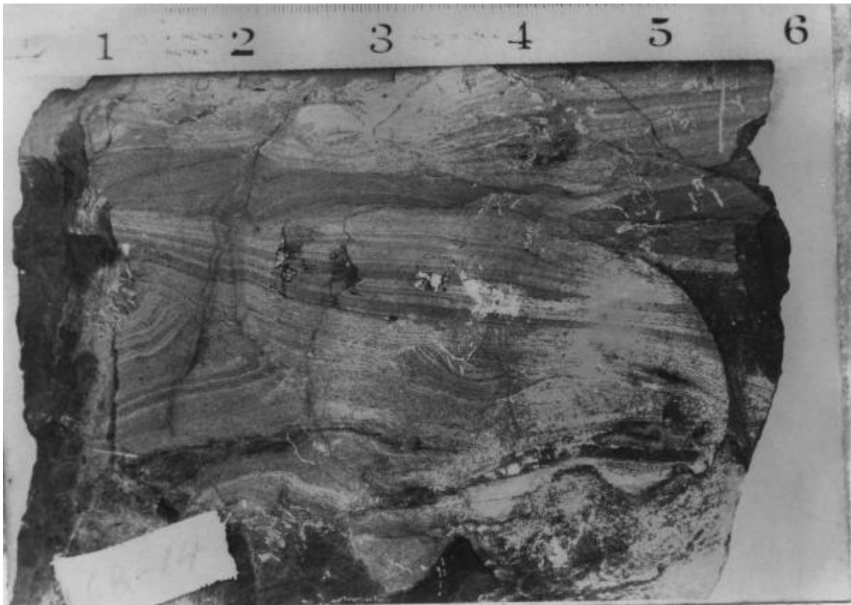
Fig. 3 - 22: Small-scale slump structures seen on the weathered surface of the shales in the St. John's Formation. The structures include slump folds and faults
