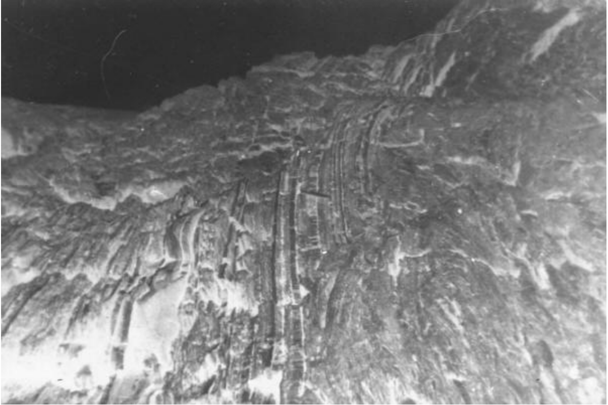
Fig. 3 - 18: Photograph exhibiting slump folds near Fishers Point. Axes of the slump folds are almost vertical and sand tumors (left bottom) are formed due to accumulation of sediments during slumping.
