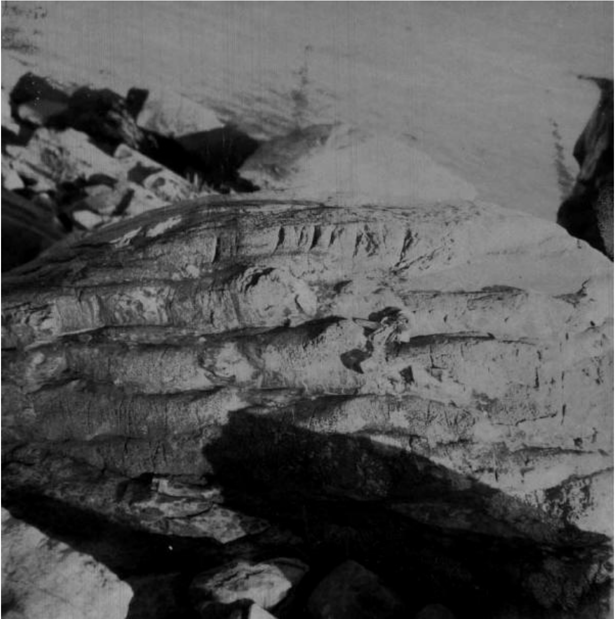
Fig. 3 - 11: Sole marks on the under surface of a graded bed in the Cape Cove Formation
