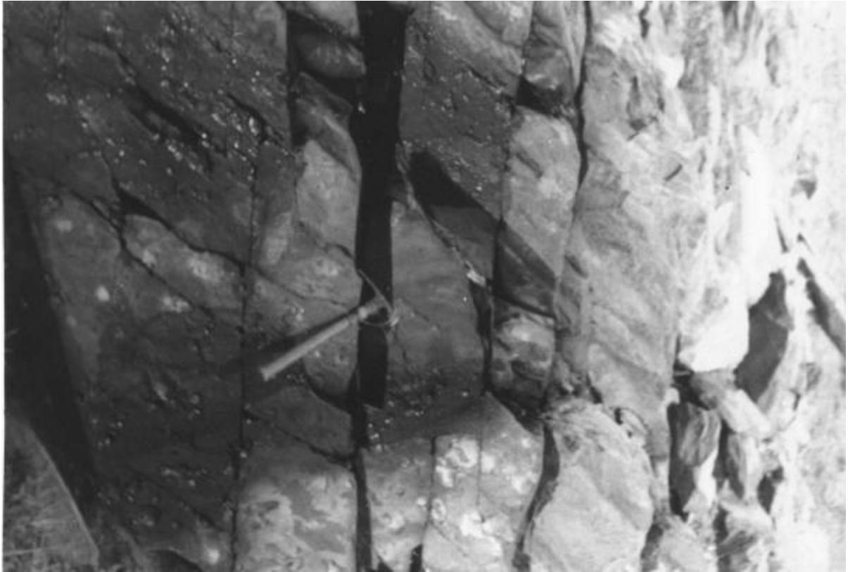
Fig. 3 - 16: Fragments produced as result of foundering in the siliceous argillites of the Freshwater Point Formation.
