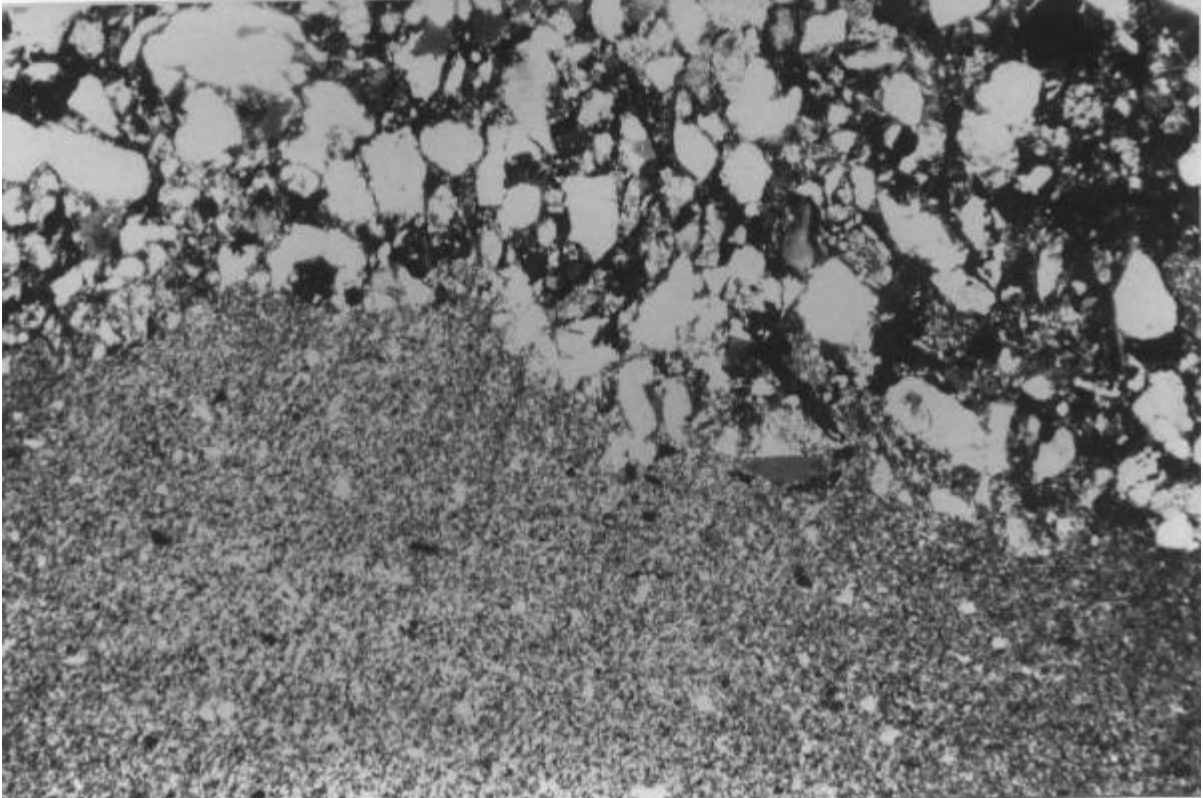
Fig. 2 - 7: Photomicrograph showing a sharp contact between two consecutive graded beds of the Cape Cove Formation. Note the dark grains of pyrite in the argillite. X32 (approx.) under crossed nicols.
