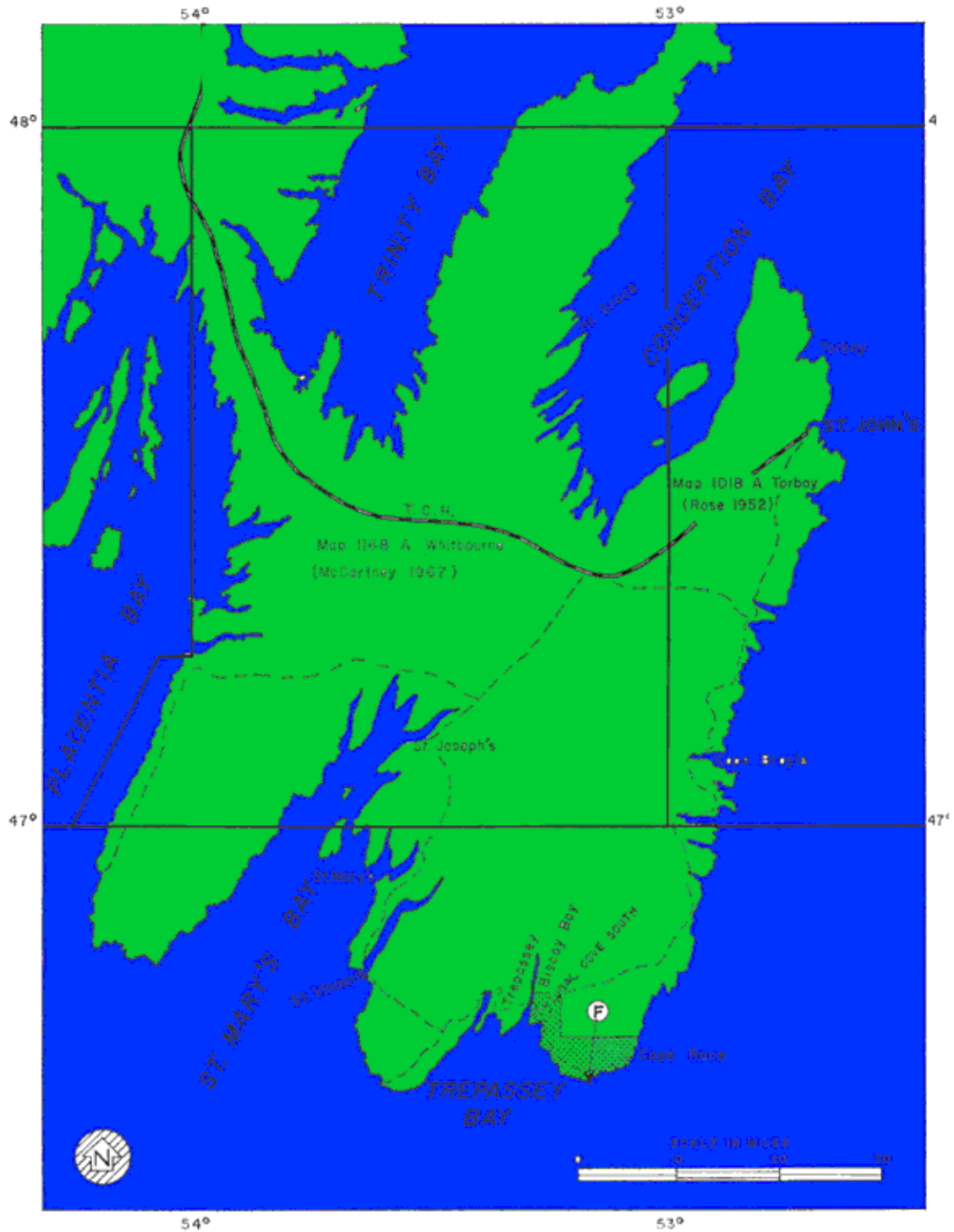
Fig. 1-1: Location map of the area showing index of previously mapped areas in the Avalon Peninsula. The area marked by dots is the Biscay Bay - Cape Race area.
