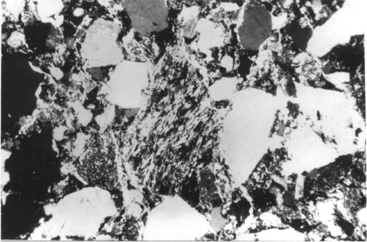
Fig. 2 - 6: Photomicrograph showing basic volcanic rock fragments in the Cape Cove greywacke. X32 (approx.) under crossed nicols.
