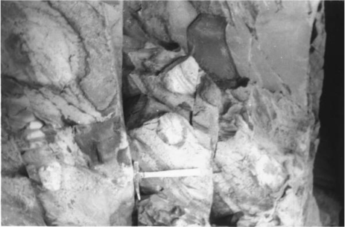
Fig. 3 - 14: Concretionary blocks of red siltstone found in the Drook cherts near Drook Point
