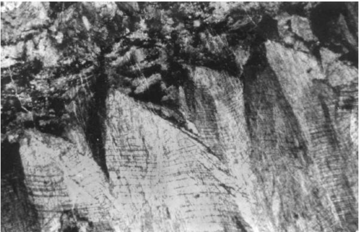
Fig. 2 - 7: Photomicrograph showing a sharp contact between two consecutive graded beds of the Cape Cove Formation. Note the dark grains of pyrite in the argillite. X32 (approx.) under crossed nicols.
