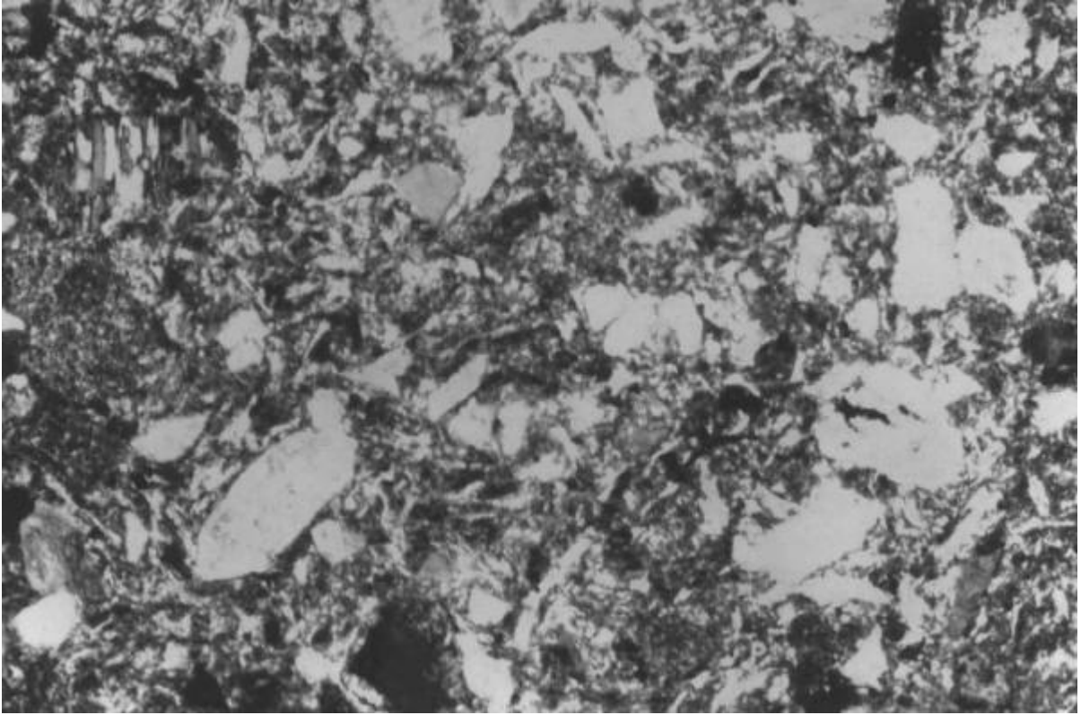
Fig. 2 - 9: Photomicrograph of volcanic tuff of the St. John's Formation showing devitrified glass (shards). X32 (approx.) under crossed nicols.
