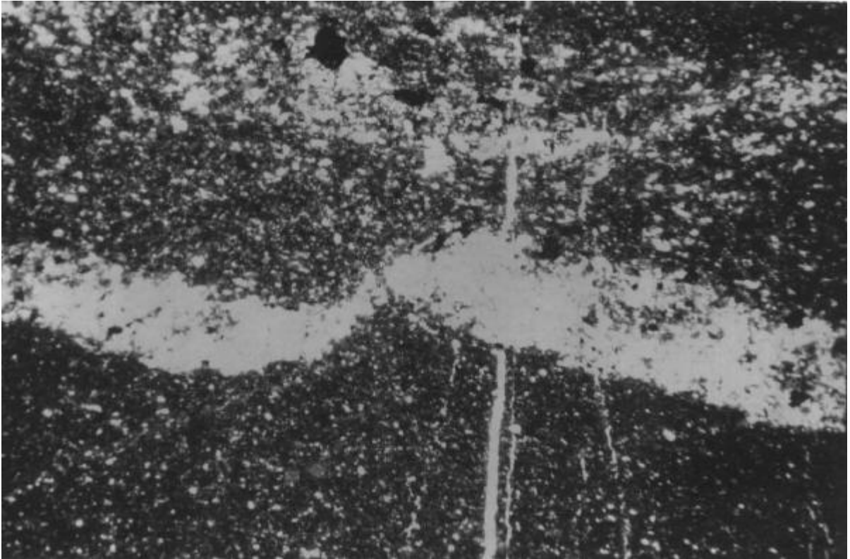
Fig. 2 - 4: Photomicrograph of Cape Cove greywacke showing quartz grains and rock fragments.
