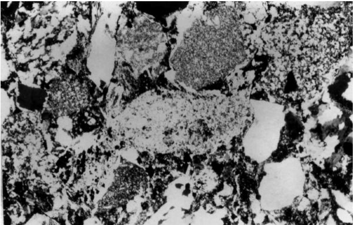
Fig. 2 - 4: Photomicrograph of Cape Cove greywacke showing quartz grains and rock fragments.
