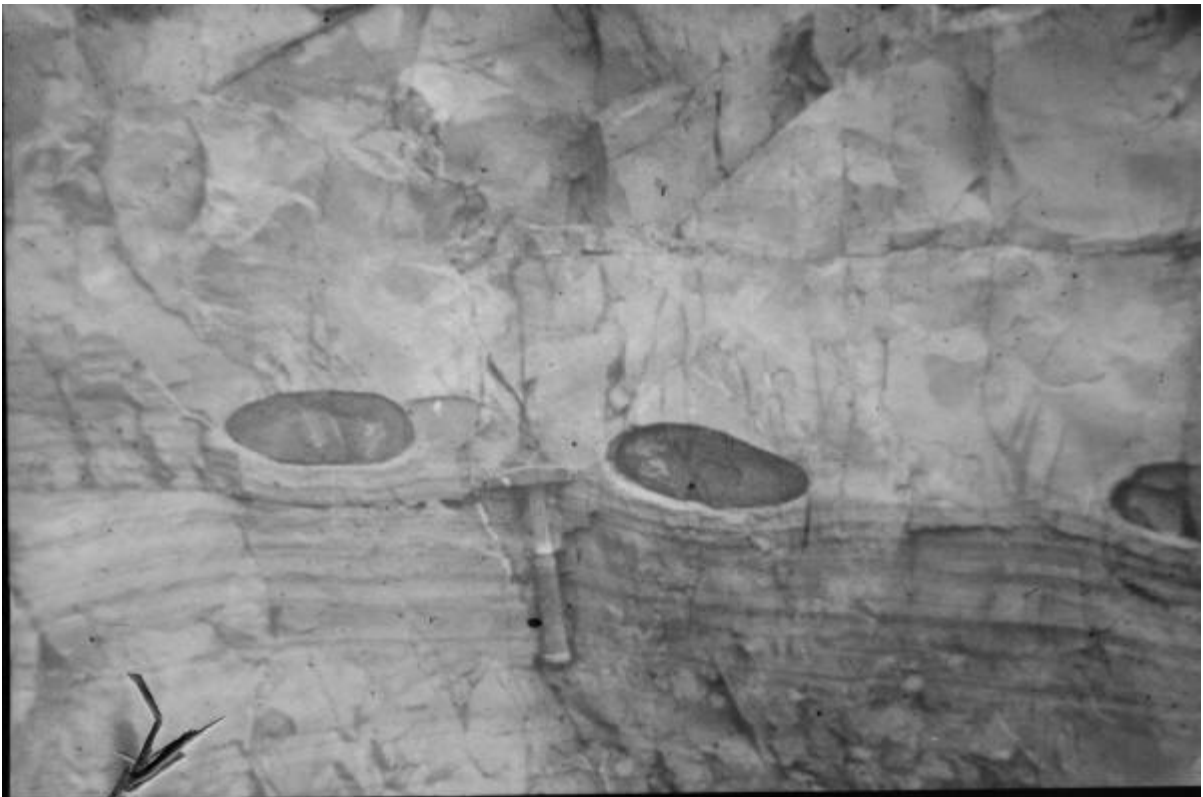
Fig. 3 - 13: Ellipsoidal calcareous sandstone nodules in banded cherts of the Drook Formation.
