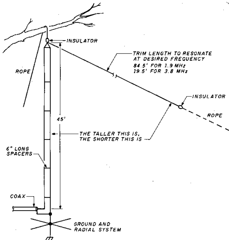
The 160/80 meter antenna at WD0P.
