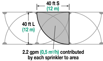
Figure 44: Square sprinkler spacing pattern with part circle sprinkler
