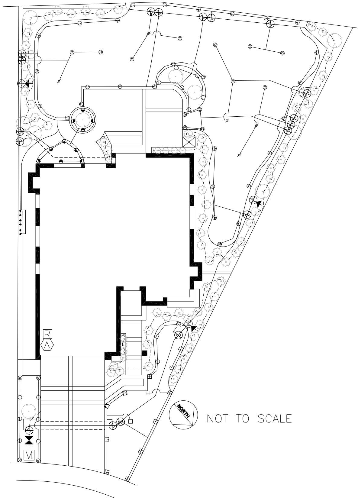
Figure 61: Plan, valve groups
