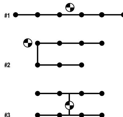
Figure 54: Split-length lateral configurations
