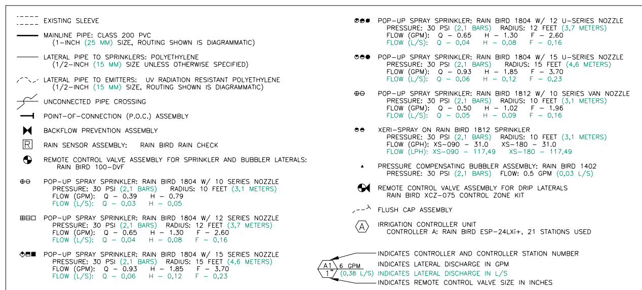
Figure 79: Irrigation legend
