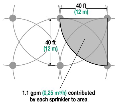
Figure 43: Square sprinkler spacing pattern with full circle sprinkler
