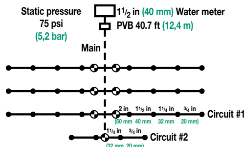
Figure 65: Piping plan
