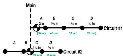
Figure 56: Deep U-shape circuits
