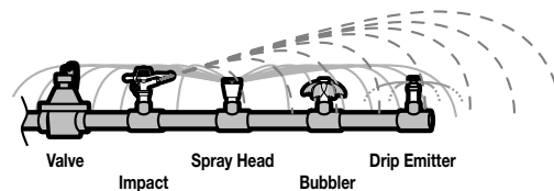
Figure 24: Avoid mixing sprinkler heads on each valve
