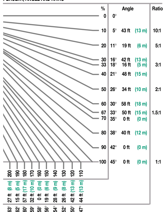
Figure 16: Slope reference
